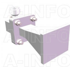
LB-90-10-C-NFSPO Standard Gain Horn Antenna 8.2-12.4GHz 10dB Gain N Type Female
