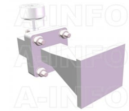
LB-90-10-C-7SPO Standard Gain Horn Antenna 8.2-12.4GHz 10dB Gain 7mm
